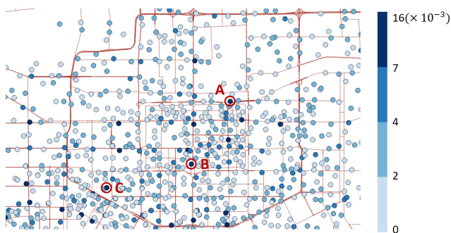
Fig. 10: Spatial distribution of PageRank centrality.
