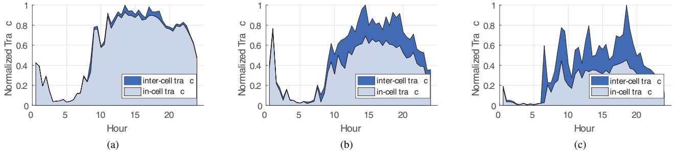
Fig. 3: An illustration of three typical in-cell and inter-cell cell tower data traffic characteristics. (a) In-cell traffic dominant, collected from a cell tower in a residential area; (b) Inter-cell traffic consistently notable during the daytime, collected from a cell tower in a shopping mall; (c) Inter-cell traffic surges at certain times, collected from a cell tower in a transit station.
