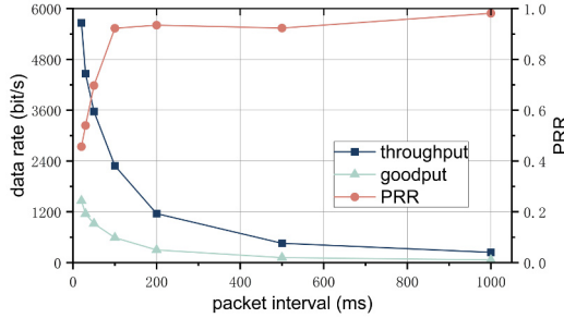
Fig. 4. Effect of transmission interval on PRR and Data rate.
