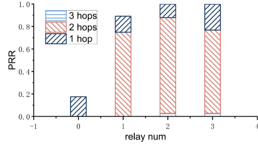
Fig. 7. Effect of relay num on PRR.
