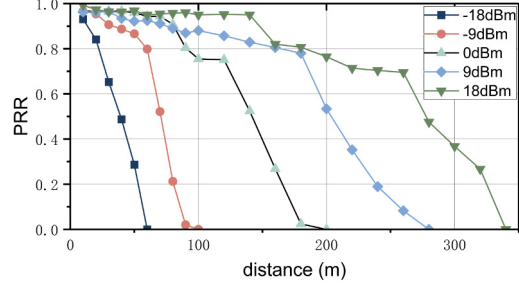
Fig. 5. Effect of TX Power on PRR.
